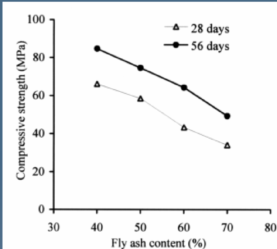
Fig. 15. Compressive strengths of concretes at 28 and 56 days.
