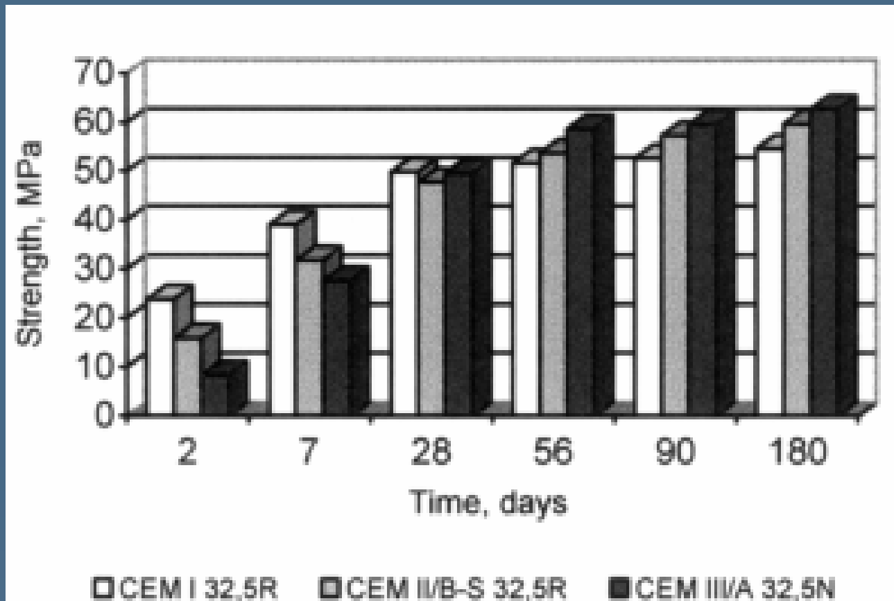
Fig. 3. Increase of cement strength CEM I 32.5R, CEM II/B-S 32.5R i CEM III/A 32.5N
